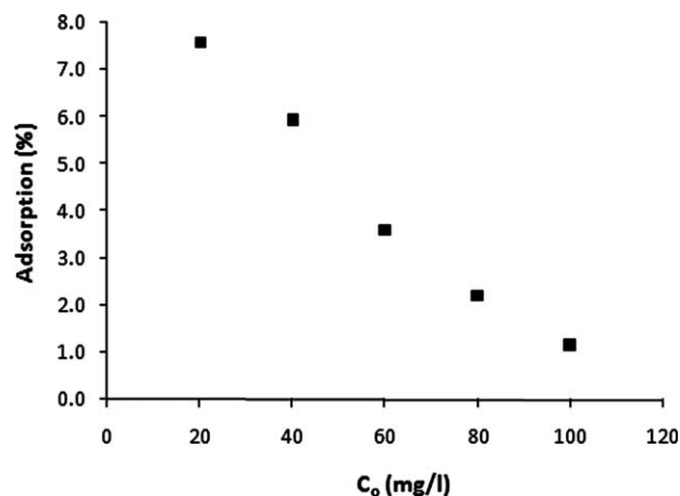
Figure 3 Effect of solution initial concentration on the adsorption of phenol on SAN polymer at T = 25^\circ\text{C} , and \text{pH} = 7 .
