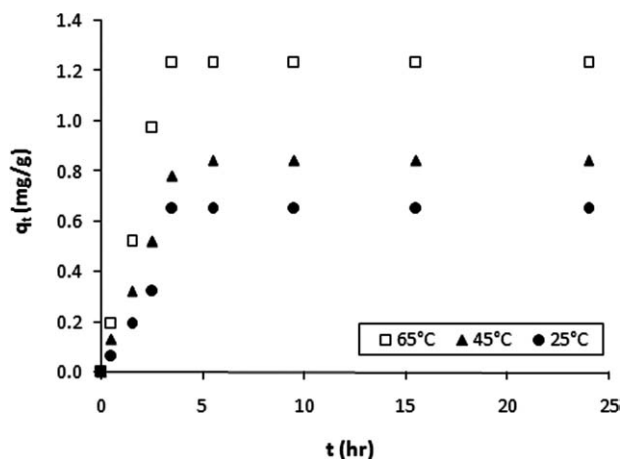
Figure 4 Effect of solution temperature on phenol adsorption on SAN polymer at C_{\text{pho}} = 40 g/L and \text{pH} = 7 .
