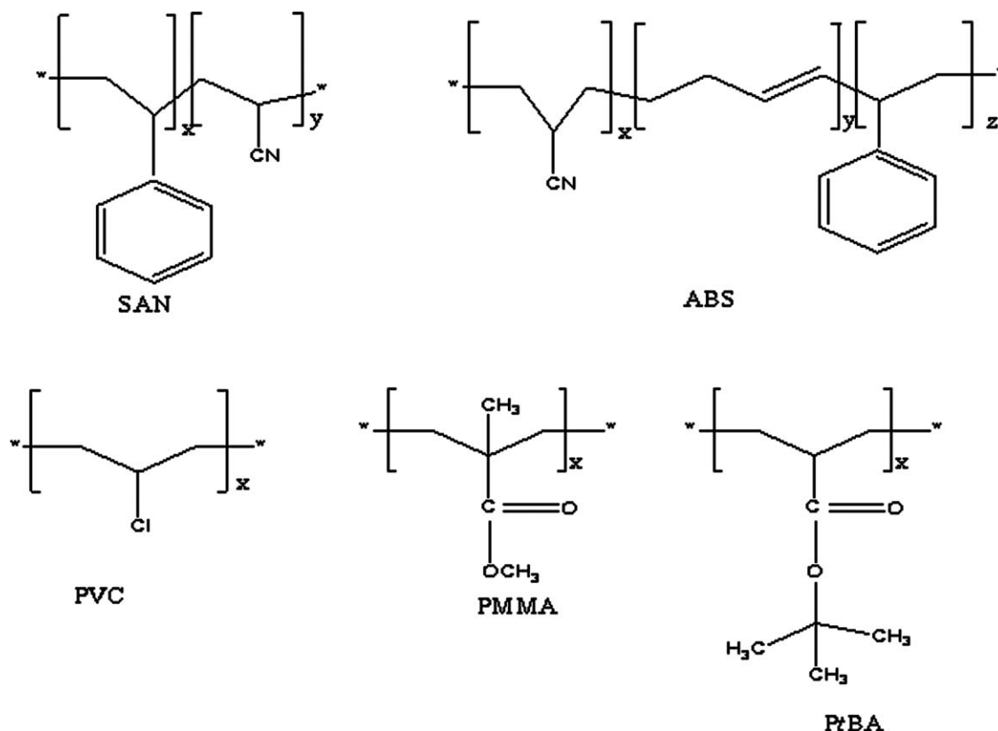
Figure 1 Structure of the polymers under study.
