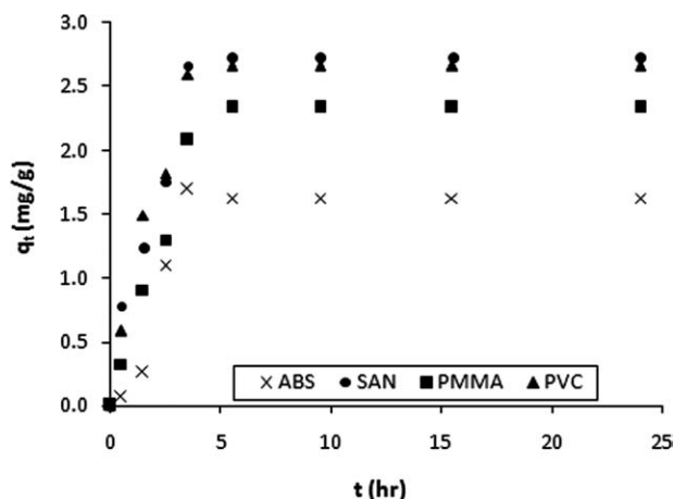
Figure 2 Effect of contact time on phenol adsorption on various polymers at C_{\text{pho}} = 40 \text{ mg/L} , T = 25^\circ\text{C} , and pH = 7 .
