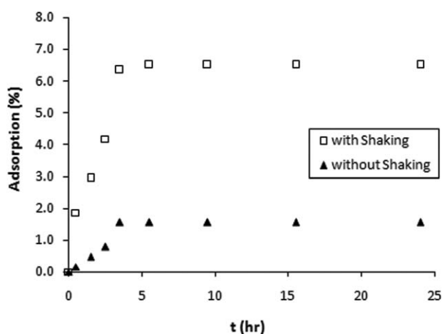
Figure 5 Effect of agitation rate on phenol adsorption on SAN polymer at T = 25^\circ\text{C} , C_{\text{pho}} = 40 g/L, and \text{pH} = 7 .
